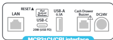
MCP31CI/CBI interface
